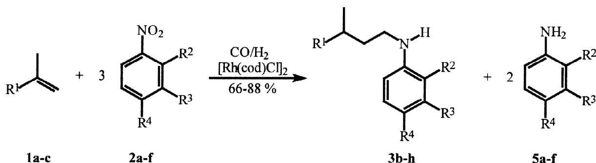
Scheme 2: Monoalkylation of aromatic nitro compounds 2a-f
