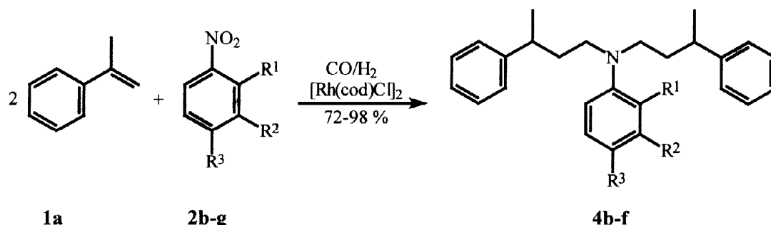
Scheme 4: Symmetrical bisalkylation of nitro compounds 2b-g with \alpha -methylstyrene ( 1a )
